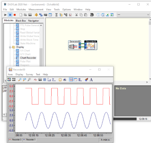
Figure 1-2. Displaying Generated Signals
