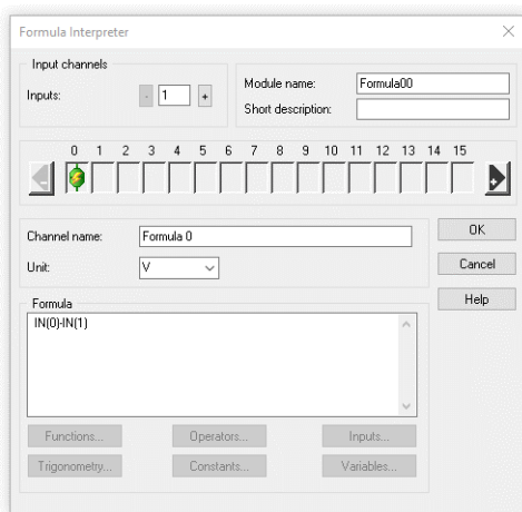
Figure 1-4. Online Calculation with the Formula Interpreter
